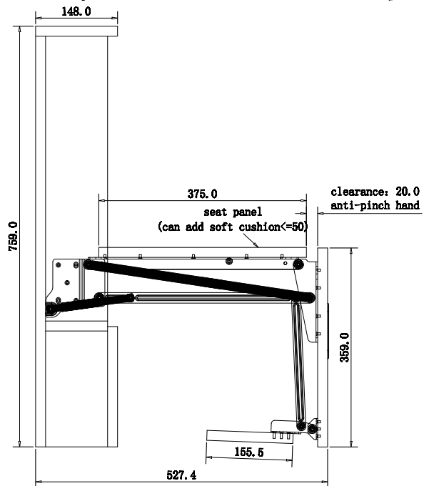
size drawing of cabinet (diagonal line of cabinet must be equal)
