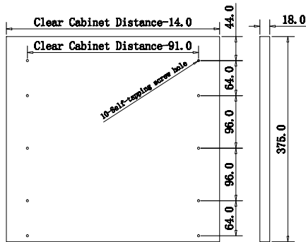
seat panel size clear cabinet distance + side panel thickness
