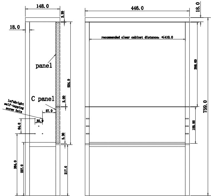
size drawing of cabinet (diagonal line of cabinet must be equal)
