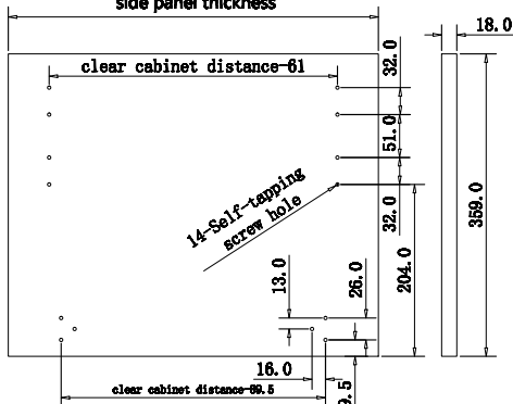
size drawing of panel
