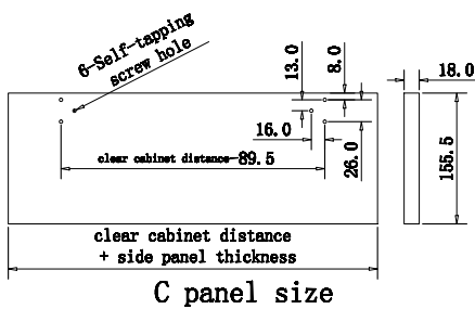
size drawing of panel
